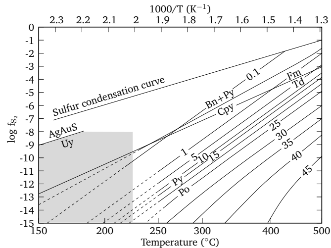
Gambar 7.2.: Diagram stabilitas mineral
