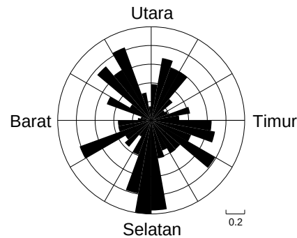
Gambar 7.8.: Contoh diagram mawar
